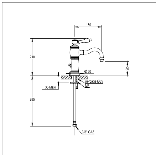
Mitigeur lavabo Julia 01.708 Single lever basin mixer 01.708
